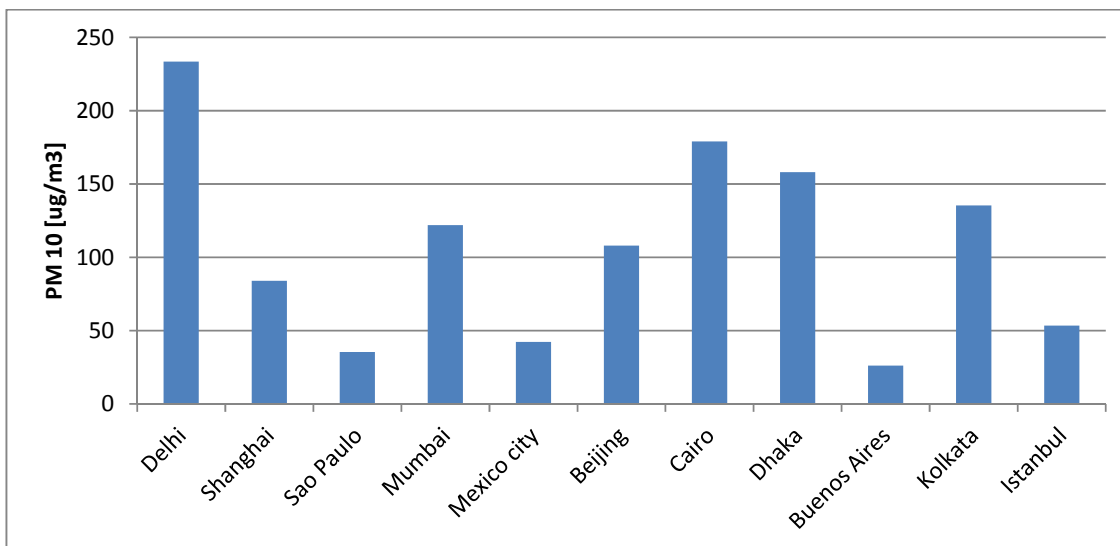
Figure 4: PM_{10} levels for available mega-cities of more than 14 million habitants for the last available year in the period 2011-2015.
