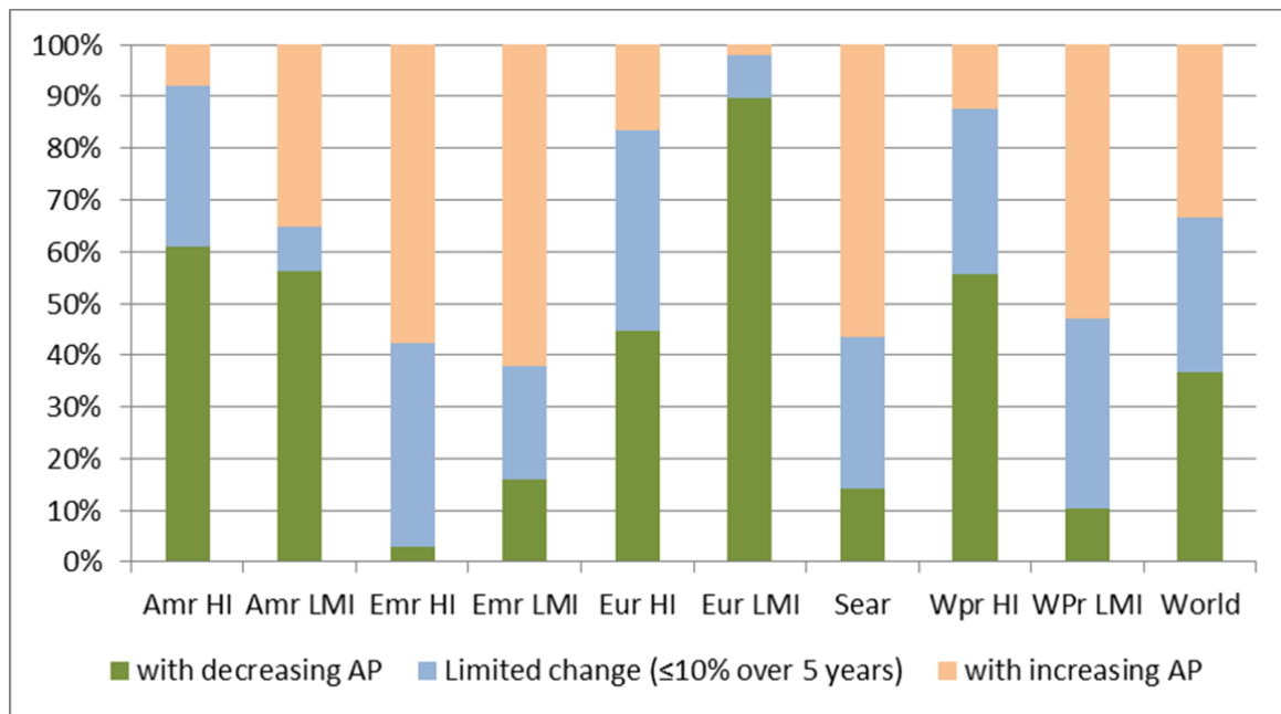
Figure 7: Percentage of city population experiencing increasing and decreasing PM 2.5 or PM 10 annual means, by region.
